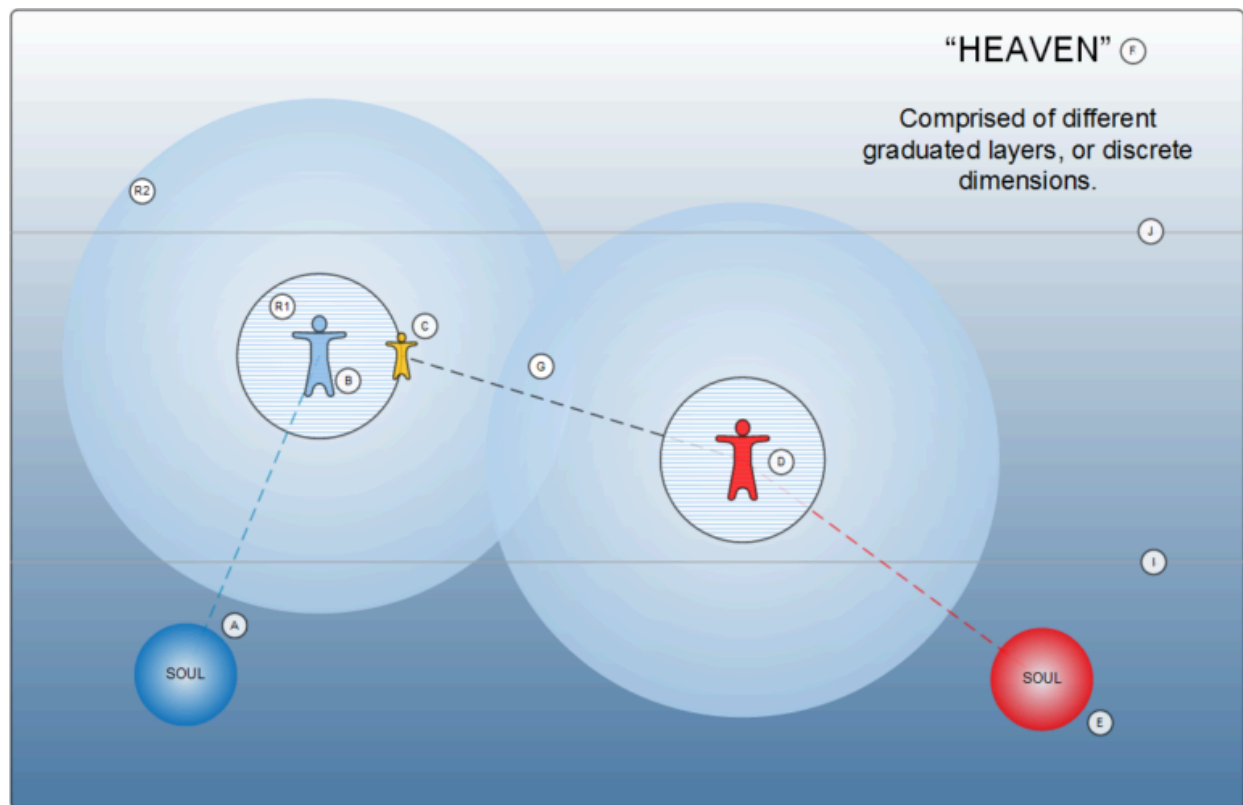
Fifth-dimensional travel as world-line travel.
